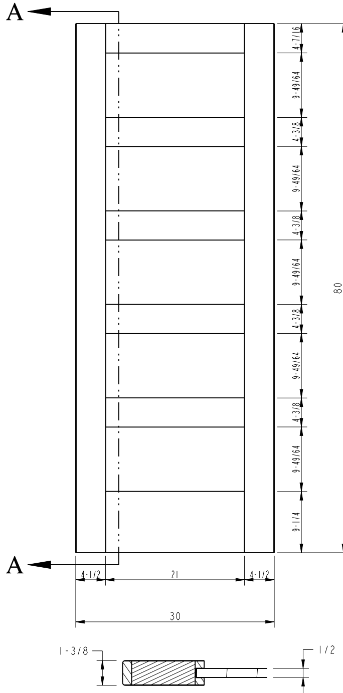
PANEL SECTION
